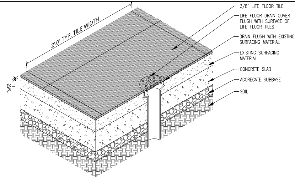
2 3/8" TILE WITH LIFE FLOOR DRAIN COVER FLUSH TO SURFACE SCALE: 1" = 1'-0"
