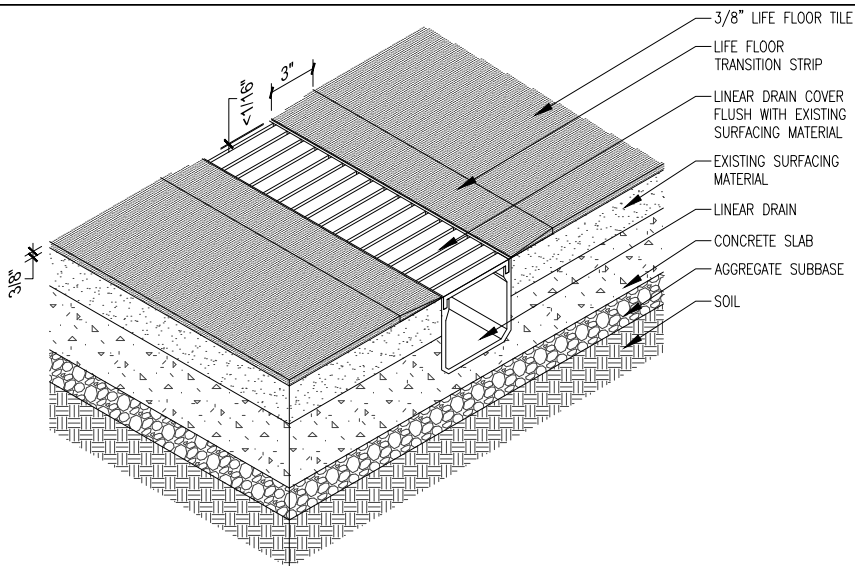
1 3/8" TILE WITH LINEAR DRAIN FLUSH TO EXISTING SURFACING MATERIAL SCALE: 1" = 1'-0"
